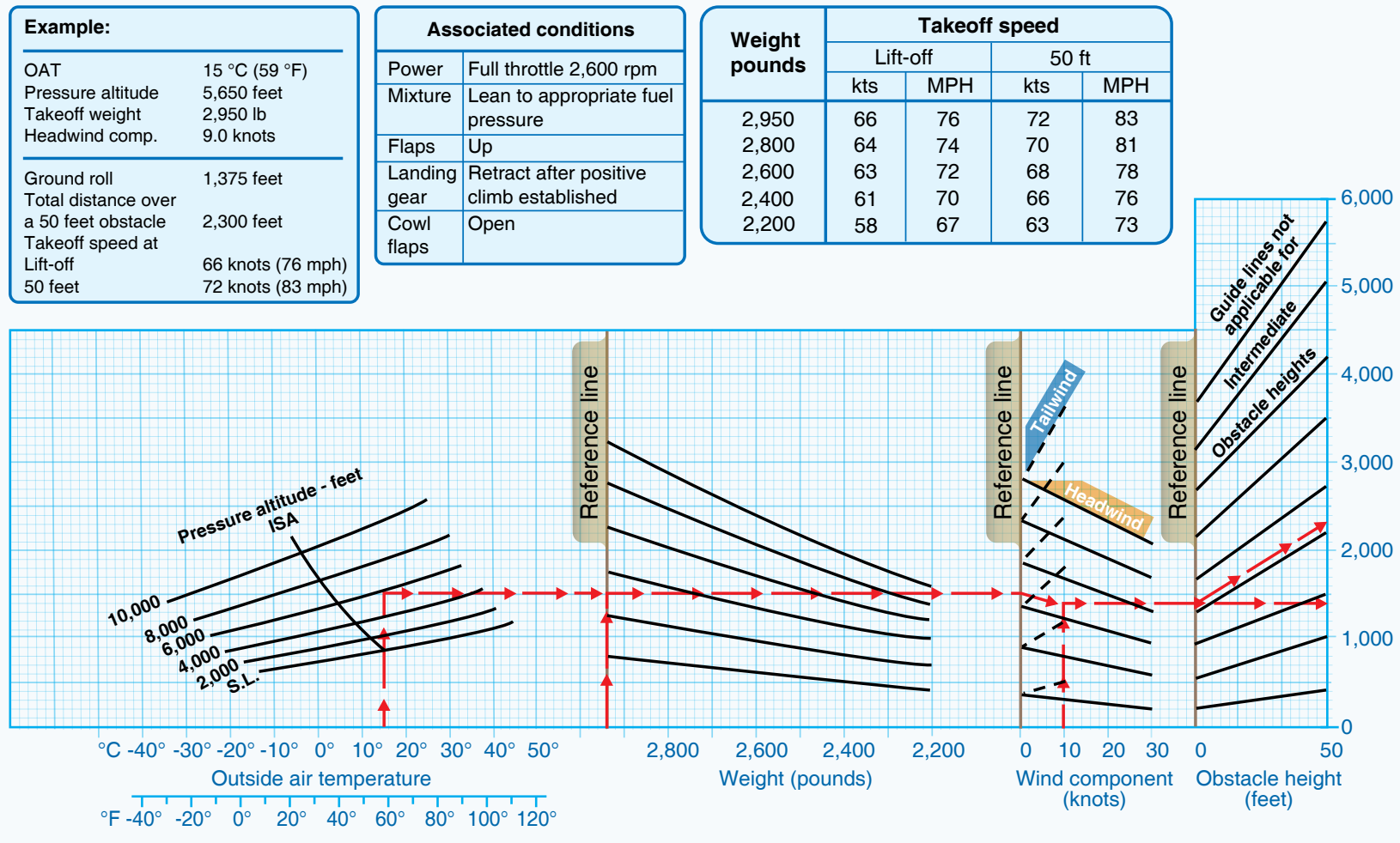
Figure 40. Airplane Takeoff Distance Graph.
